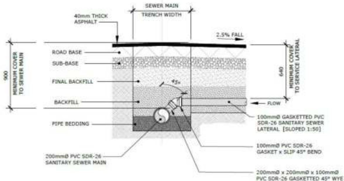
Figure 3-42 Standard sanitary sewer service connection for mains and laterals between 0.90m and 2.40m deep
