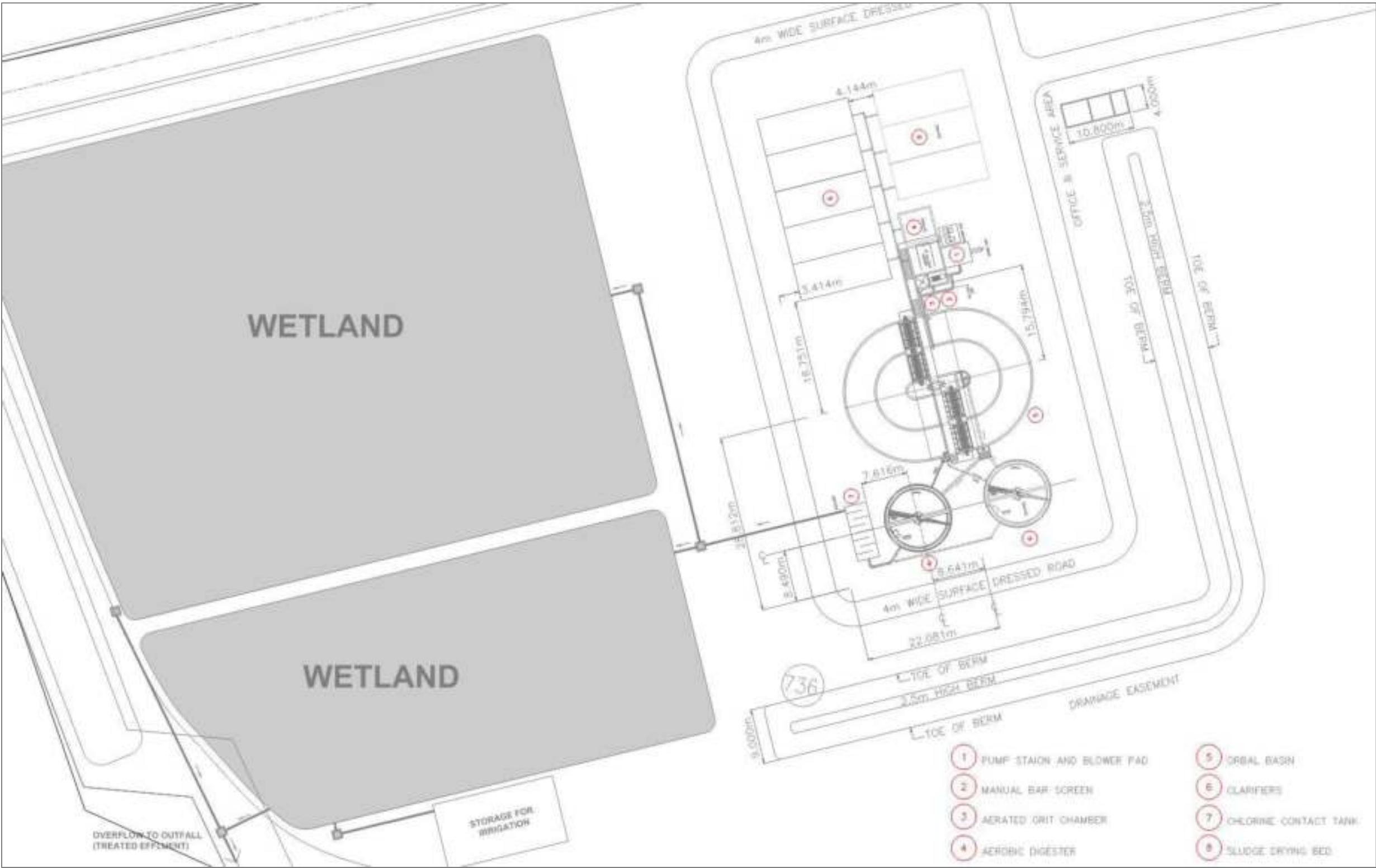
Figure 3-30 Layout of WWTP components
