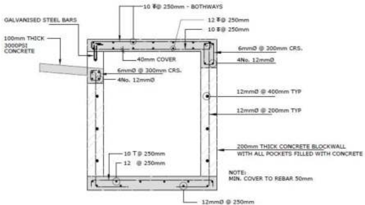
Figure 3-33 Cross-section through storm drain inlet
