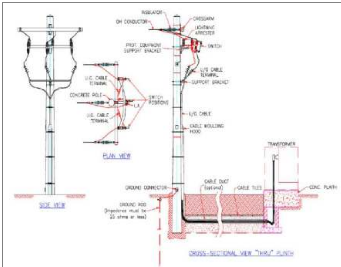
Figure 3-37 Code compliant connection methodology for transitioning of overhead 24kV, 3Φ, medium voltage distribution to underground 24kV, 3Φ medium voltage distribution
