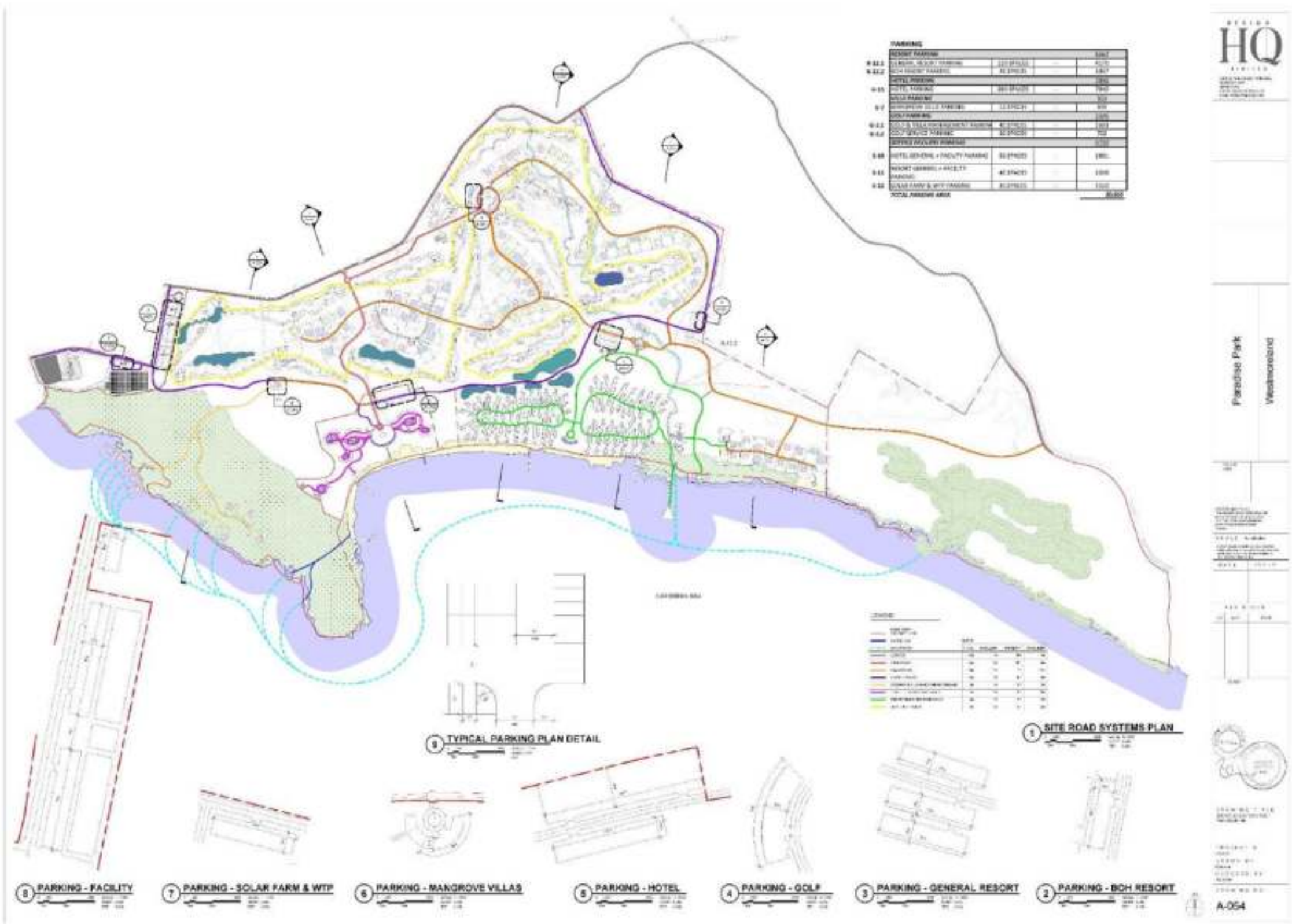
Figure 3-21 Proposed site road systems and parking plan
