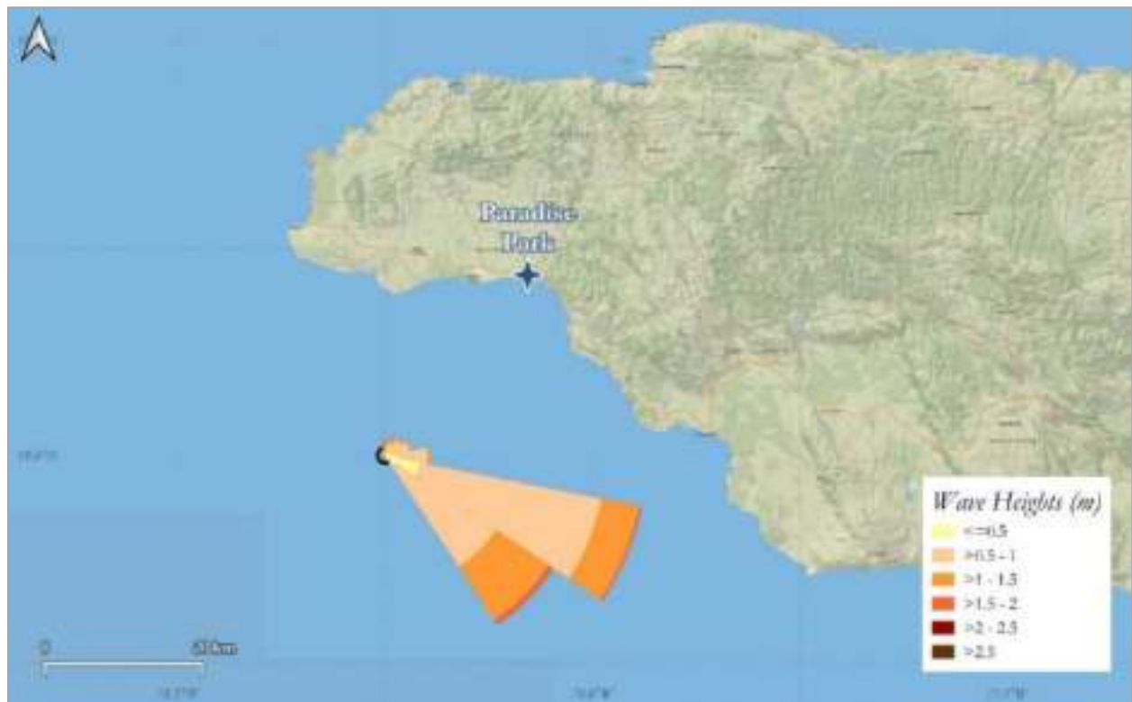
Figure 4-30 Offshore node location with wave rose showing wave heights and directions.
